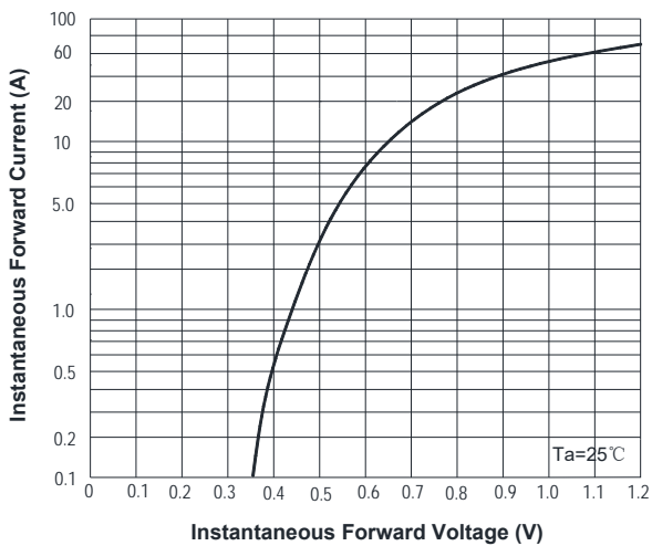
FIG3: Forward Voltage
